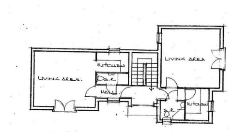
FOUR FLATS - REFUSED - FIRST FLOOR
